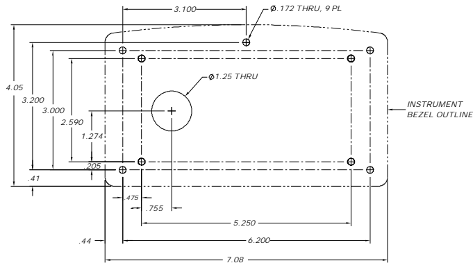
FIG. 1 PANEL HOLE DIMENSIONS
