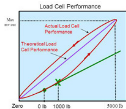
A 1000 lb test weight(s) added to set the Span
