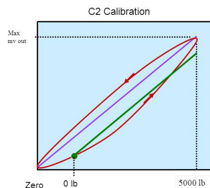
A Calibration is performed by a push of a button or a digital command
