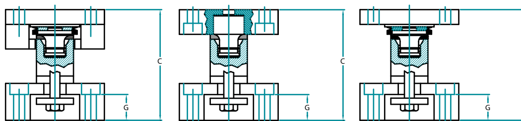
2-Directional Bumper Module (B) Fixed Loading Pin Module (F) Free Sliding Module (B)
